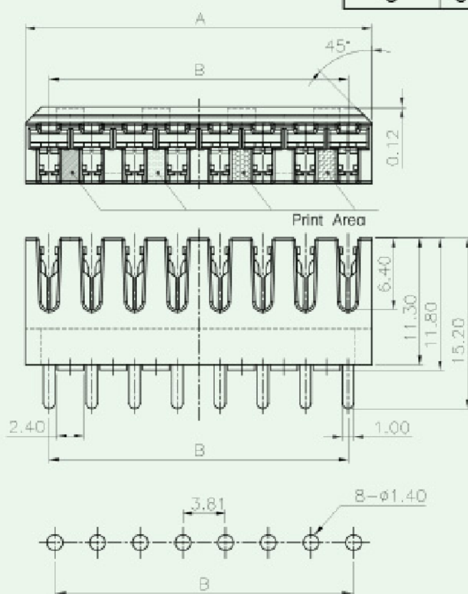
PCB Layout
