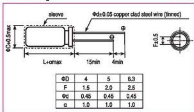
Outline Drawing
